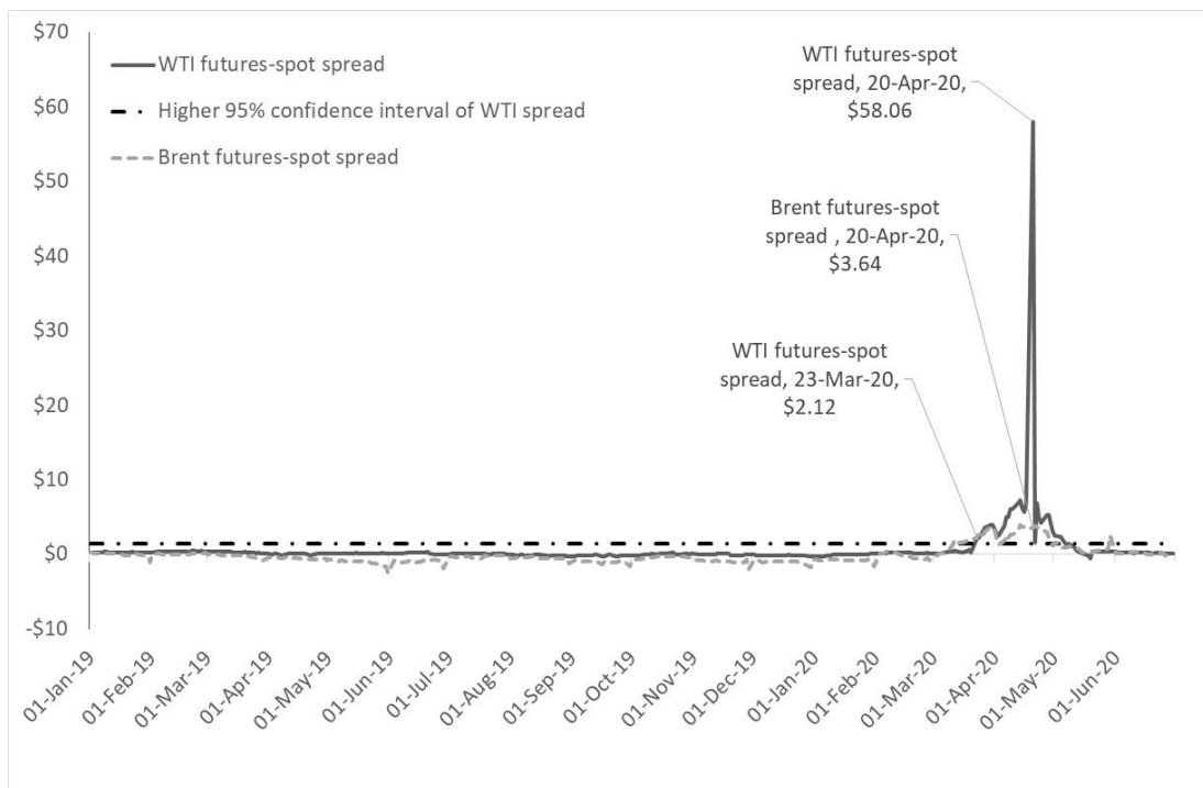
Panel B: Evolution of futures-spot spreads
