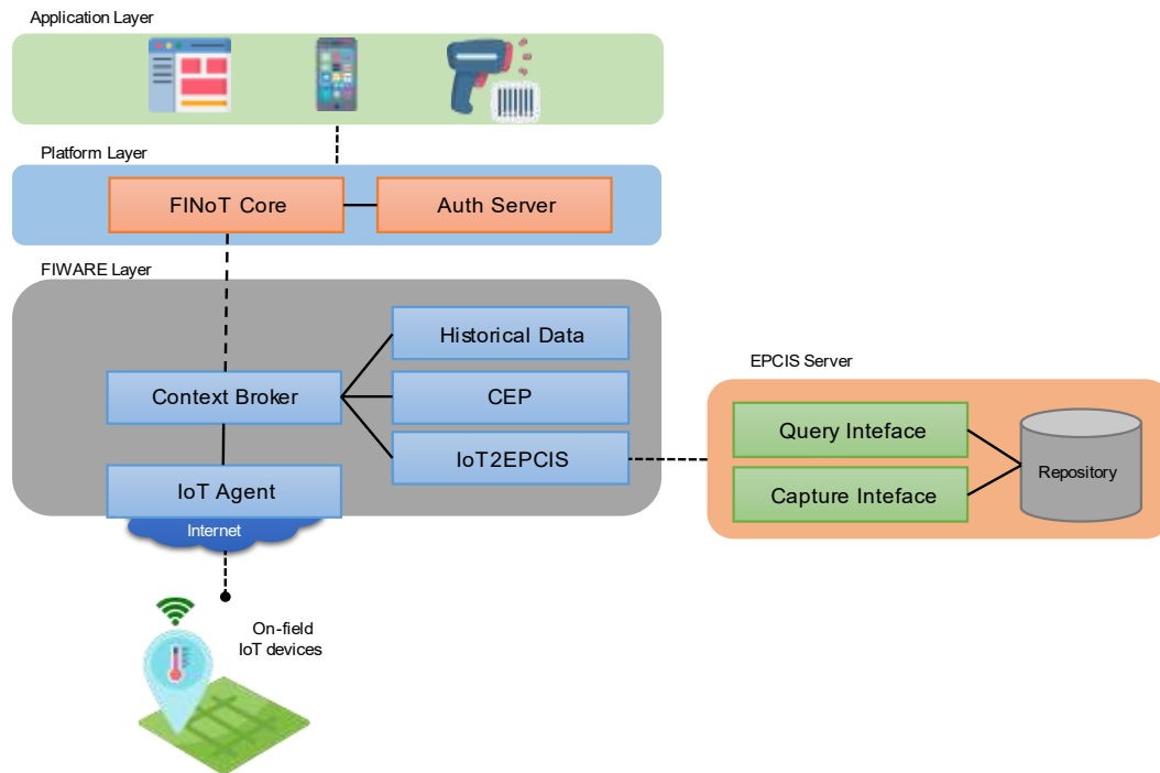
Figure 2. Conceptual Architecture
