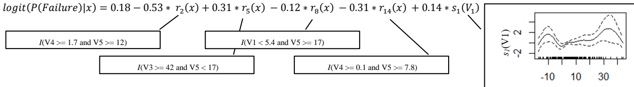
Figure 2: Illustration of the spline-rule ensemble training algorithm through application on a simplified data set.
