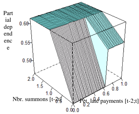
Figure 6: Graphical representation of partial dependence plots for 3 most important interaction effects
